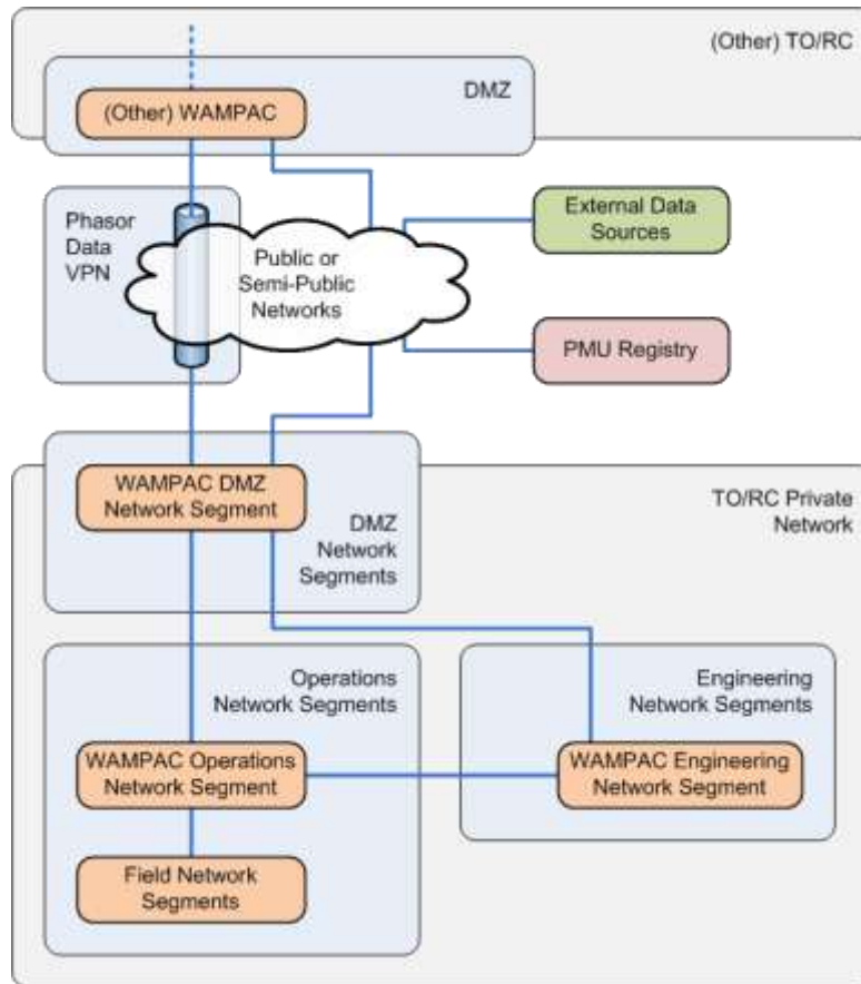
Figure 7 – Network Segmentation
