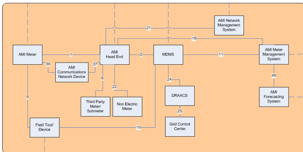
Figure 2: AMI Logical Architectural View (Internal Perspective)
